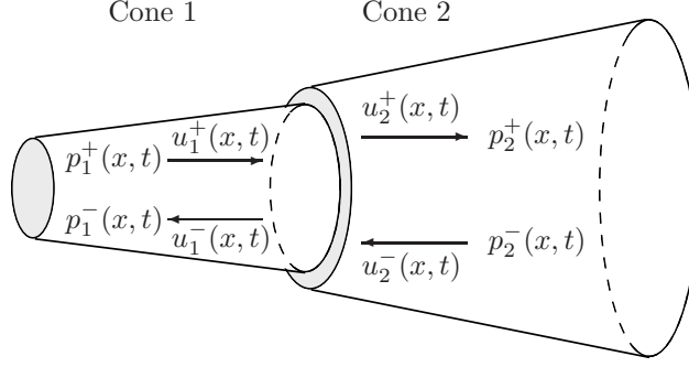
Figure 10: Junction of two conical tube sections.
