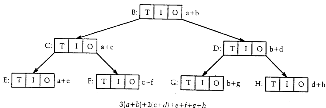
Fig. 7. The general case of MIDI interconnection forms a binary tree. The left branches receive MIDI input only from the root of the tree via MIDI THRU, and they respond to their own controls. Right
